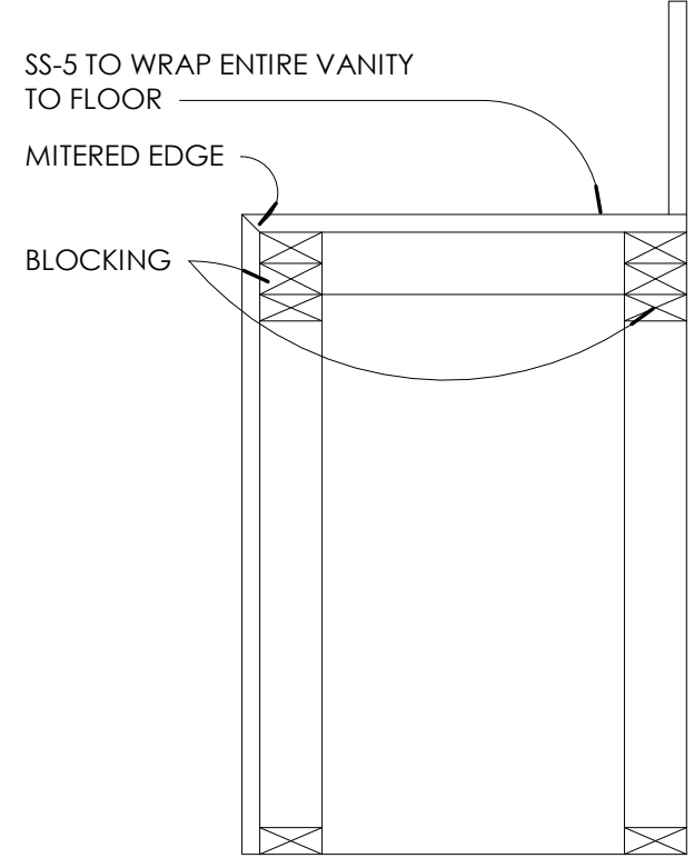
7 POWDER BATH VANITY DETAIL A 1" = 1'-0"
