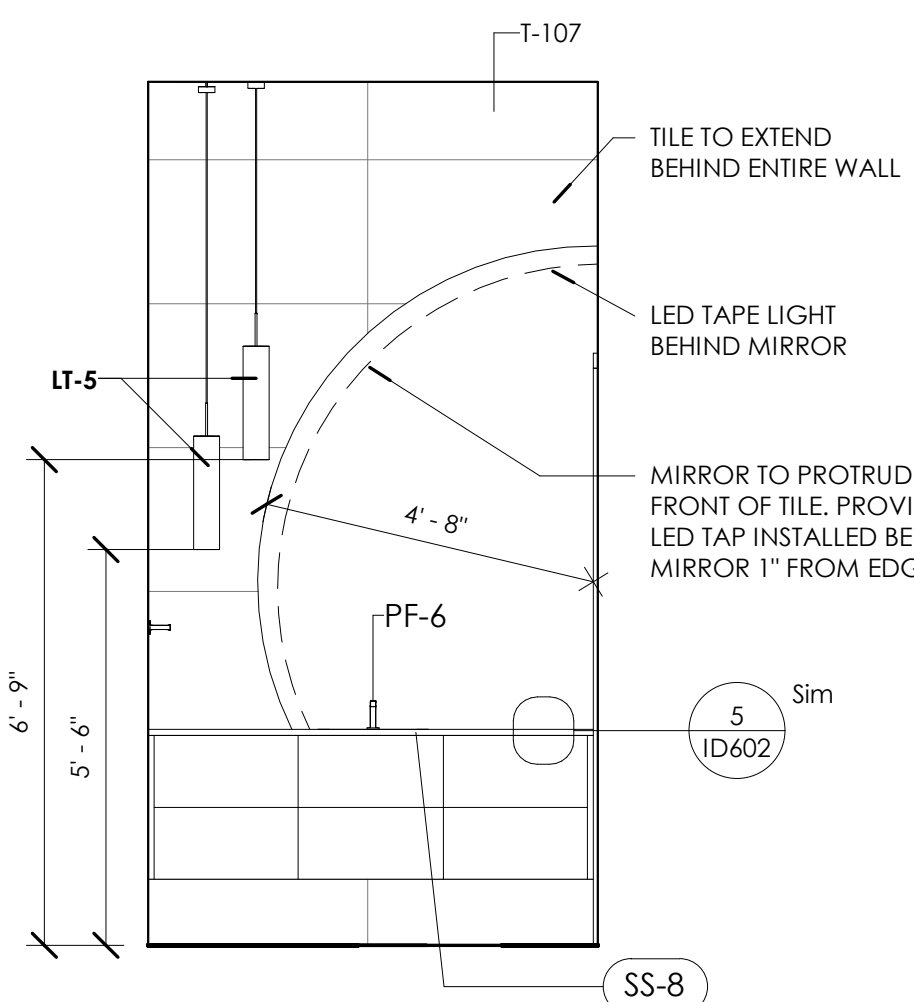
4 HIS BATH A 3/8" = 1'-0"
