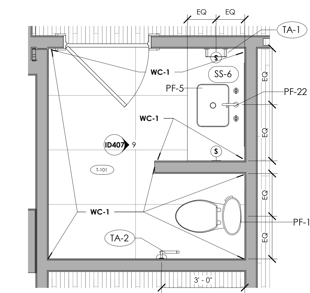
10 LEVEL 1 - POOL BATH 1/2" = 1'-0"
