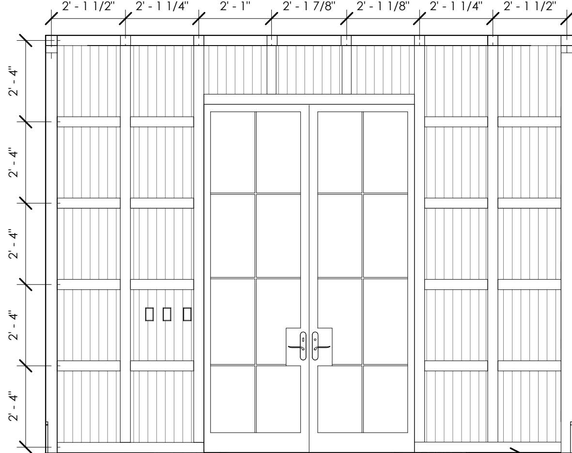
7 FOYER B 3/8" = 1'-0"
