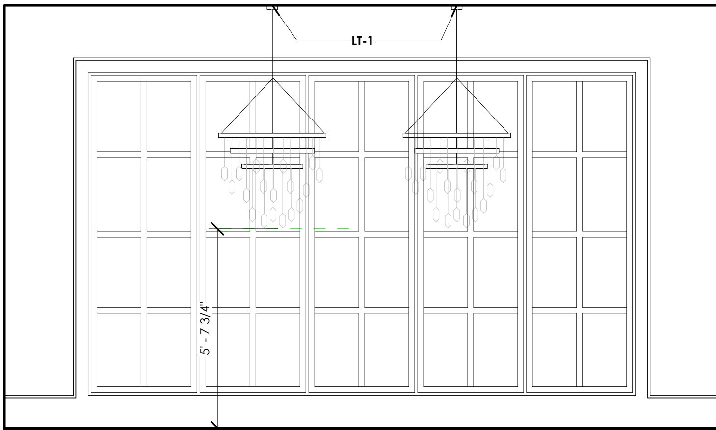
2 DINING ROOM B 3/8" = 1'-0"
