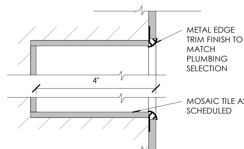
7 NICHE DETAIL 6" = 1'-0"
