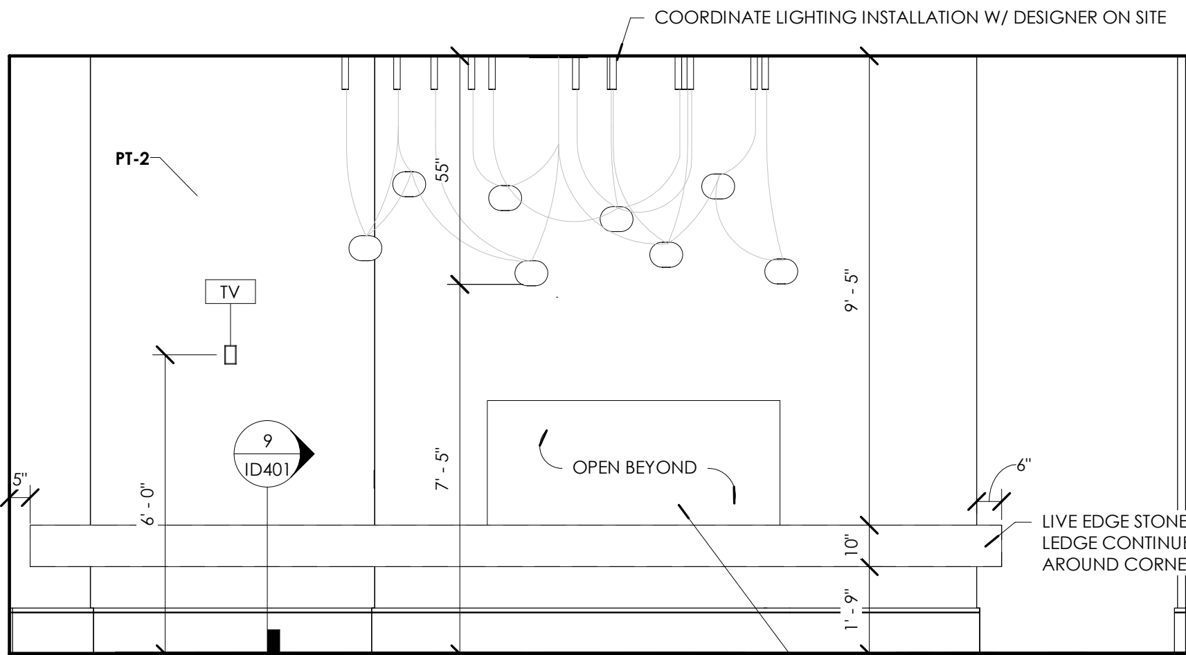
4 FIREPLACE B 3/8" = 1'-0"
