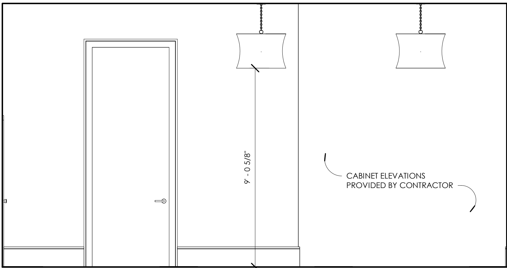
3 FRIEND'S ENTRY 3/8" = 1'-0"
