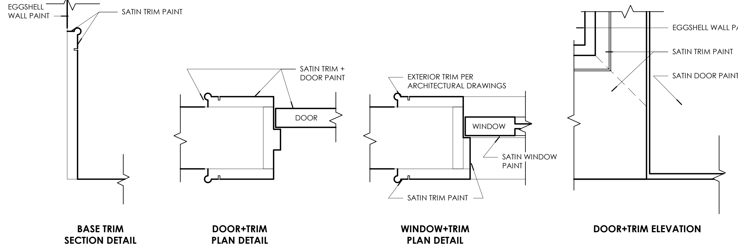
6 PAINT DETAILS 3" = 1'-0"
