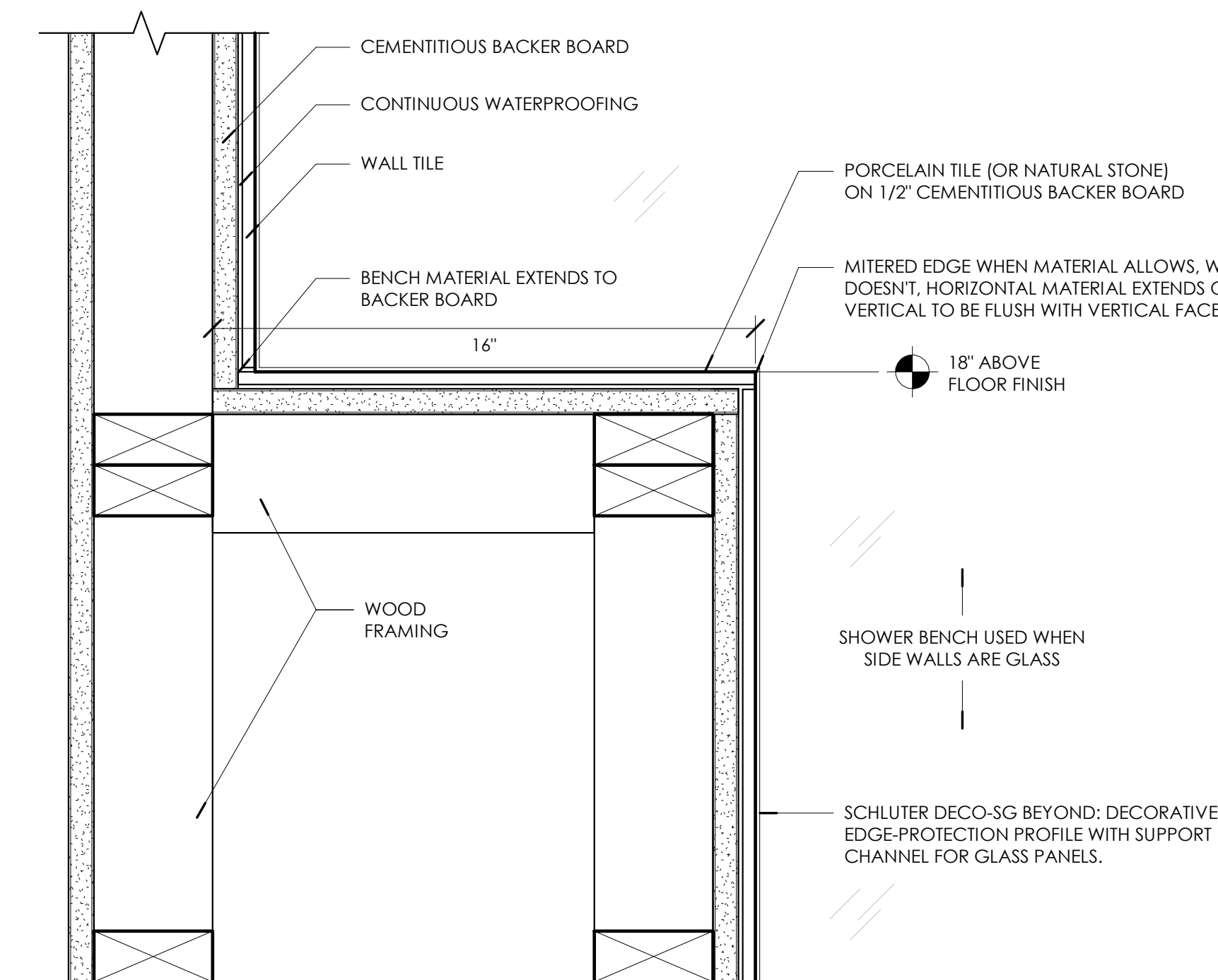
SHOWER BENCH 3" = 1'-0"
