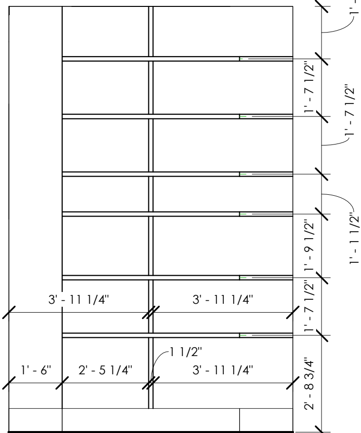
7 PANTRY B 3/8" = 1'-0"
