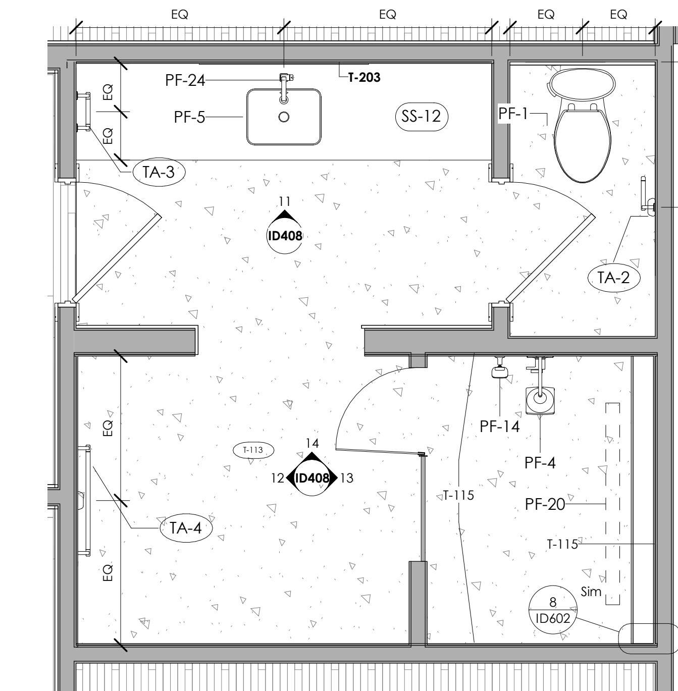
10 LEVEL 2 - GUEST BATH 2 1/2" = 1'-0"
