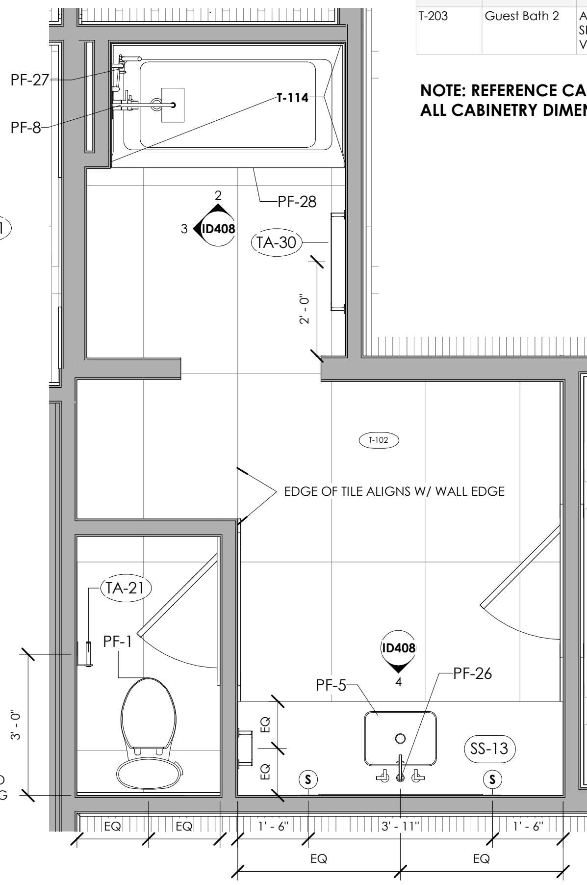
1 LEVEL 2 - GUEST BATH 1/2" = 1'-0"
