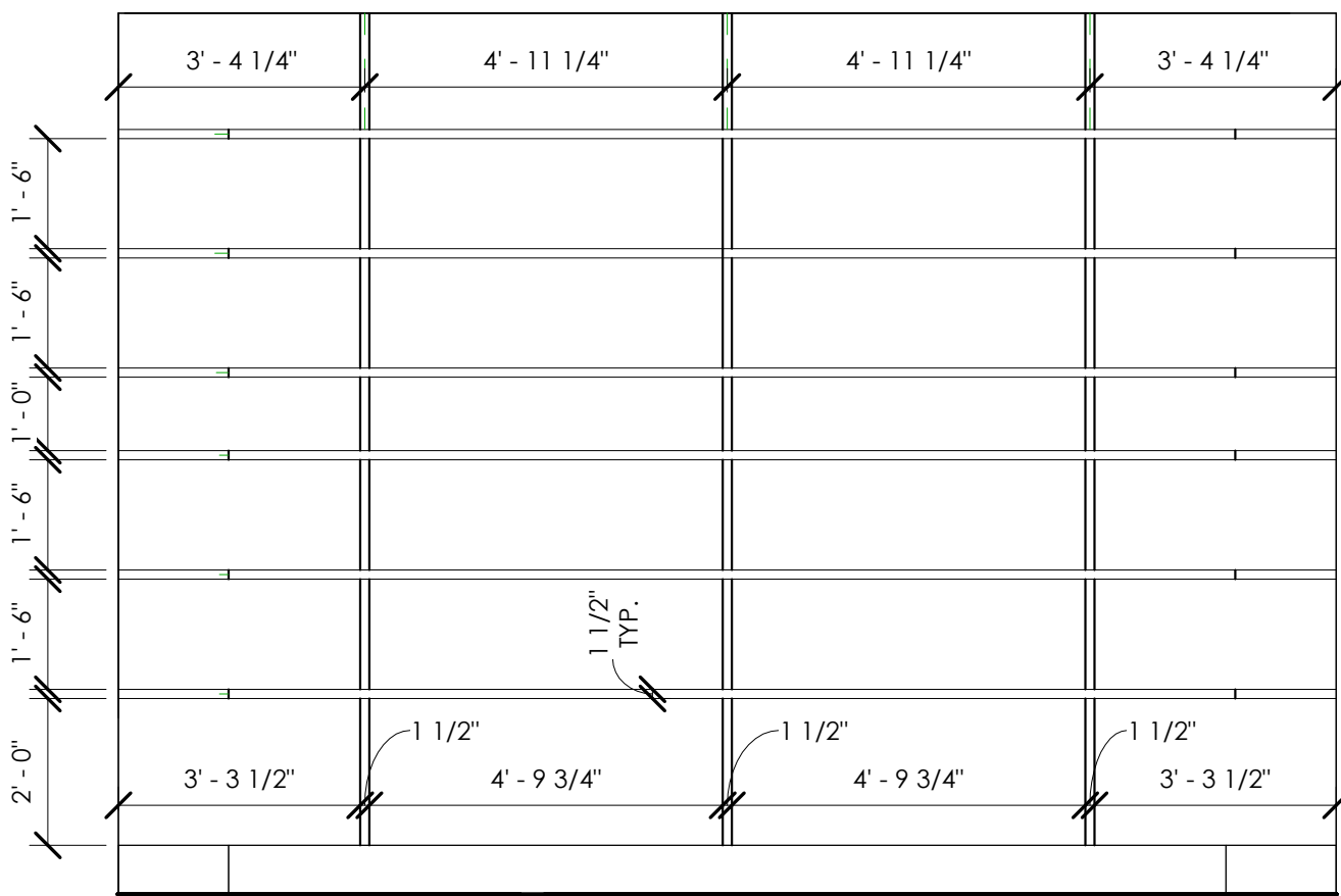
8 PANTRY A 3/8" = 1'-0"
