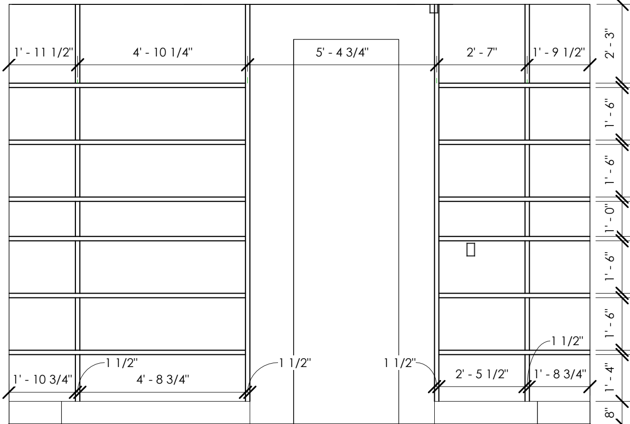
5 PANTRY D 3/8" = 1'-0"
