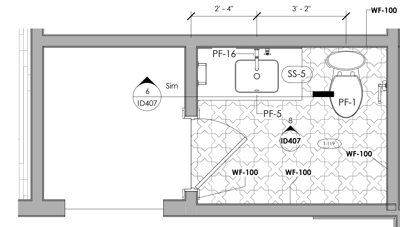
5 LEVEL 1 - POWDER BATH 1/2" = 1'-0"
