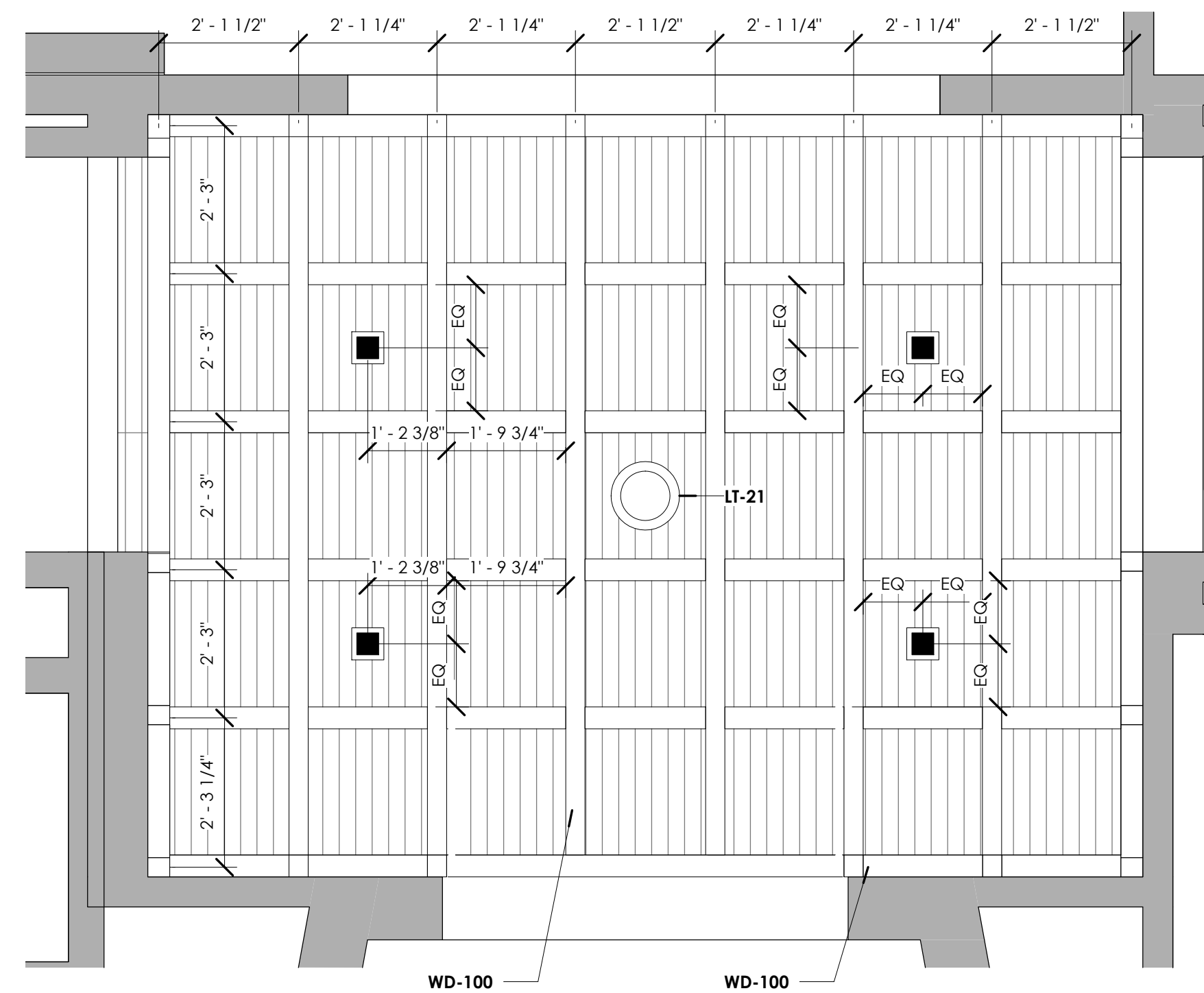
3 LEVEL 1 FOYER CEILING ENLARGED PLAN 1/2" = 1'-0"
