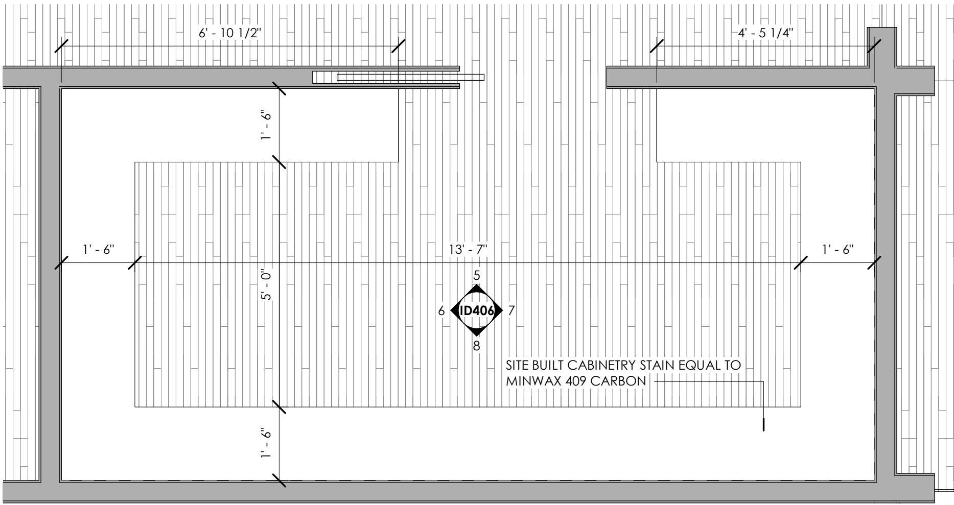
9 LEVEL 1 - PANTRY 1/2" = 1'-0"
