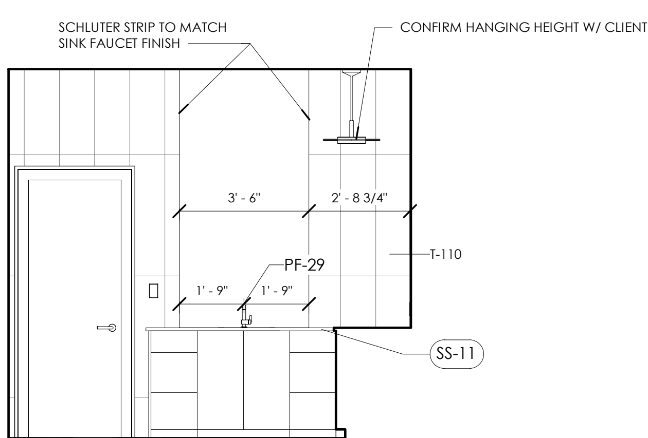
7 GUEST BATH 3 D 3/8" = 1'-0"
