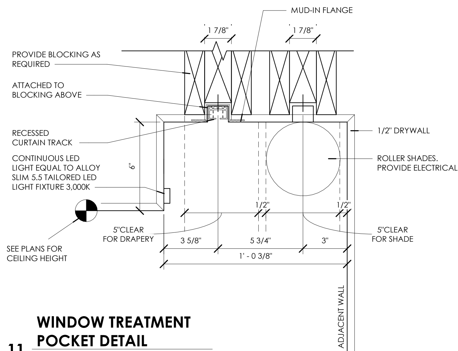
WINDOW TREATMENT POCKET DETAIL - CURTAIN ONLY 3" = 1'-0"
