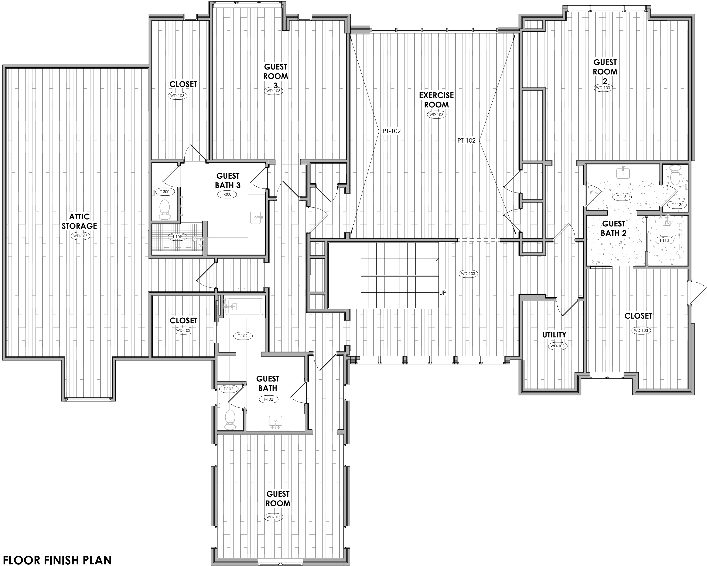
1 LEVEL 2 FLOOR FINISH PLAN 3/16" = 1'-0"
