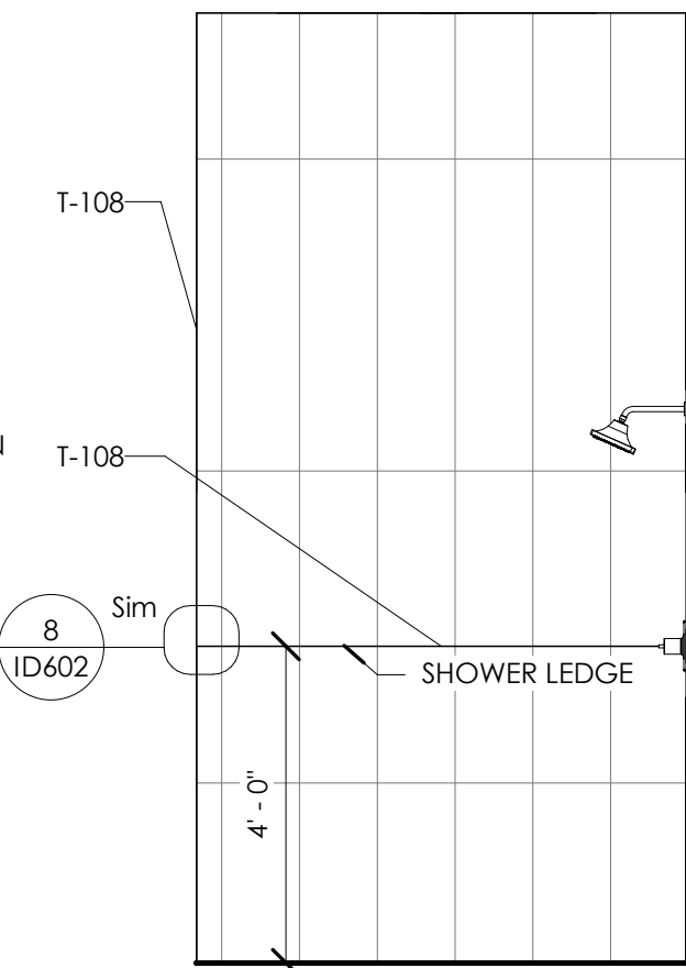
3 HIS BATH B 3/8" = 1'-0"
