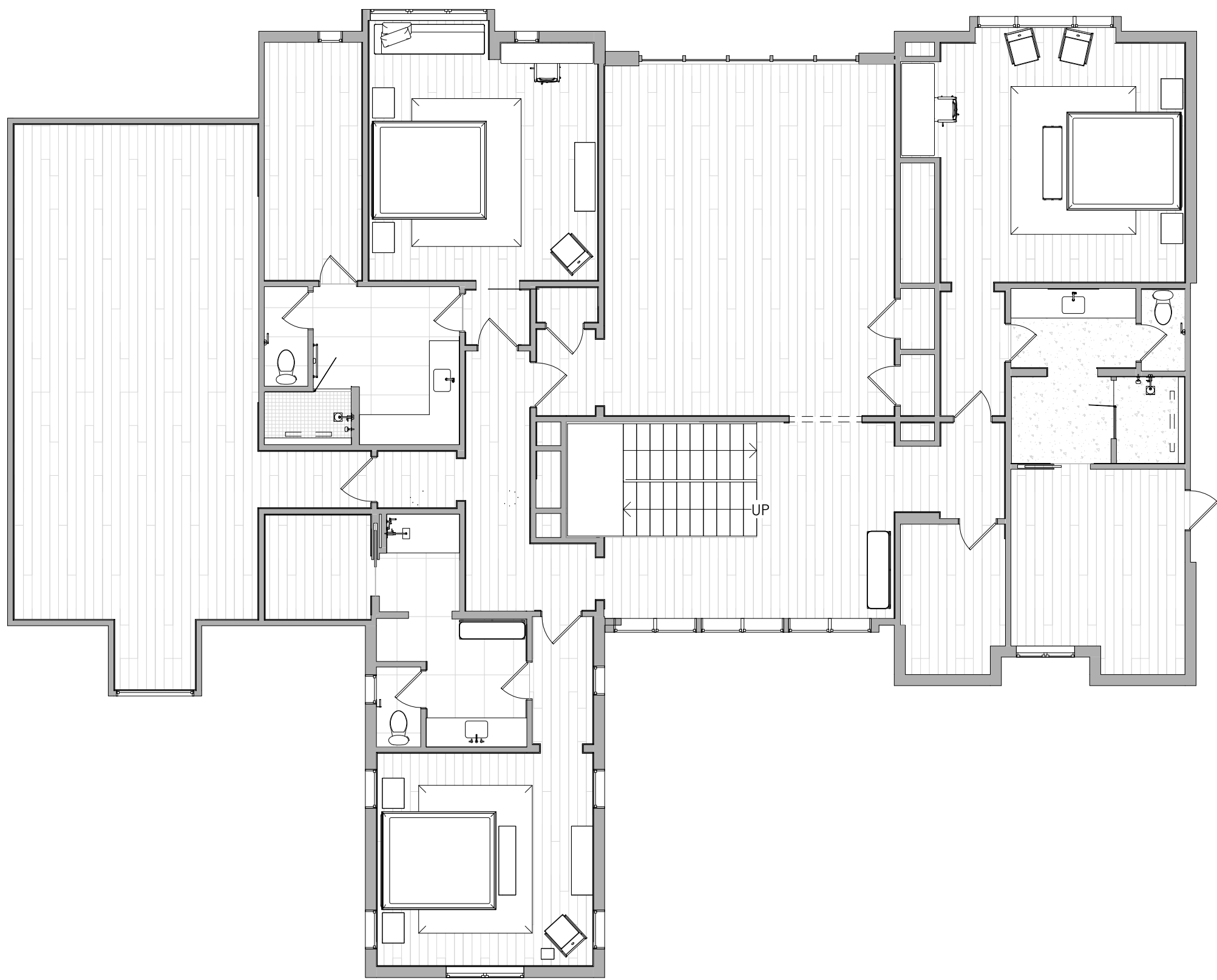
2 LEVEL 2 FURNITURE PLAN 1/8" = 1'-0"
