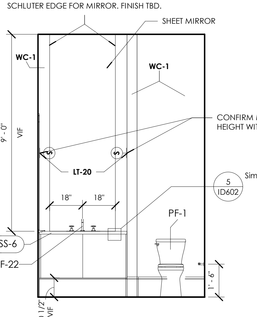
9 POOL BATH 3/8" = 1'-0"
