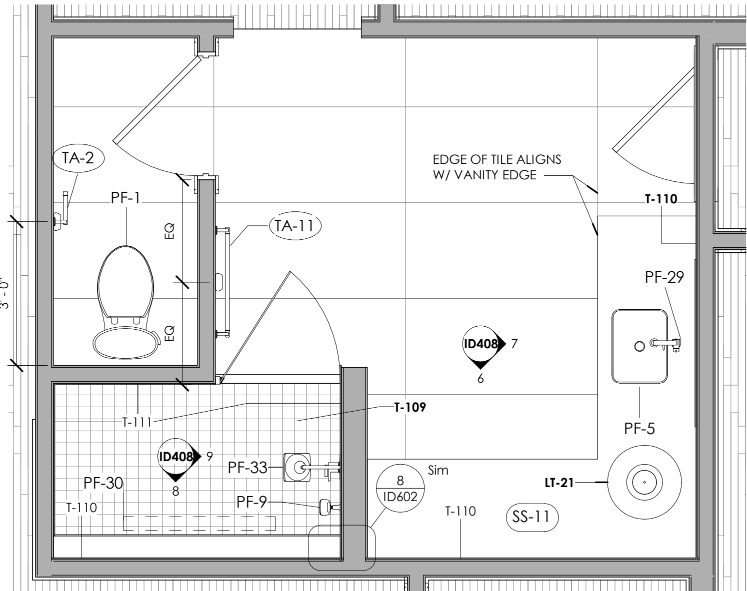
5 LEVEL 2 - GUEST BATH 3 1/2" = 1'-0"
