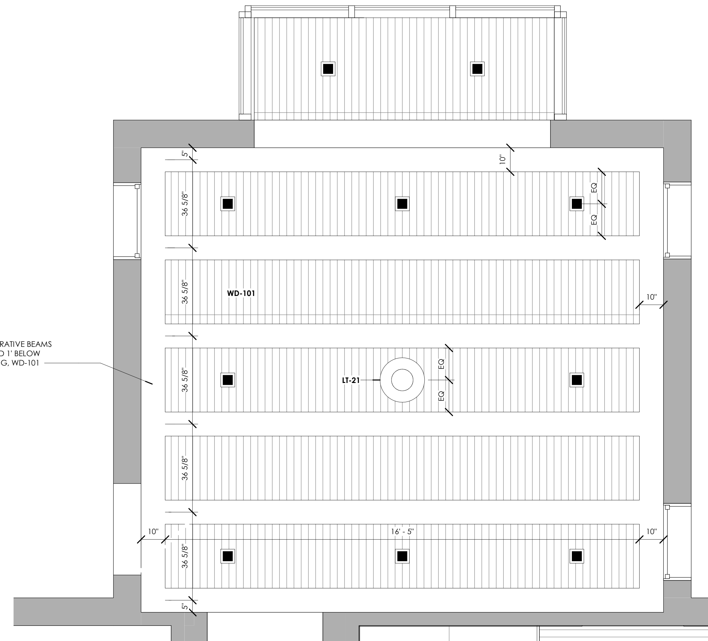
4 LEVEL 1 MASTER BEDROOM CEILING ENLARGED PLAN 1/2" = 1'-0"
