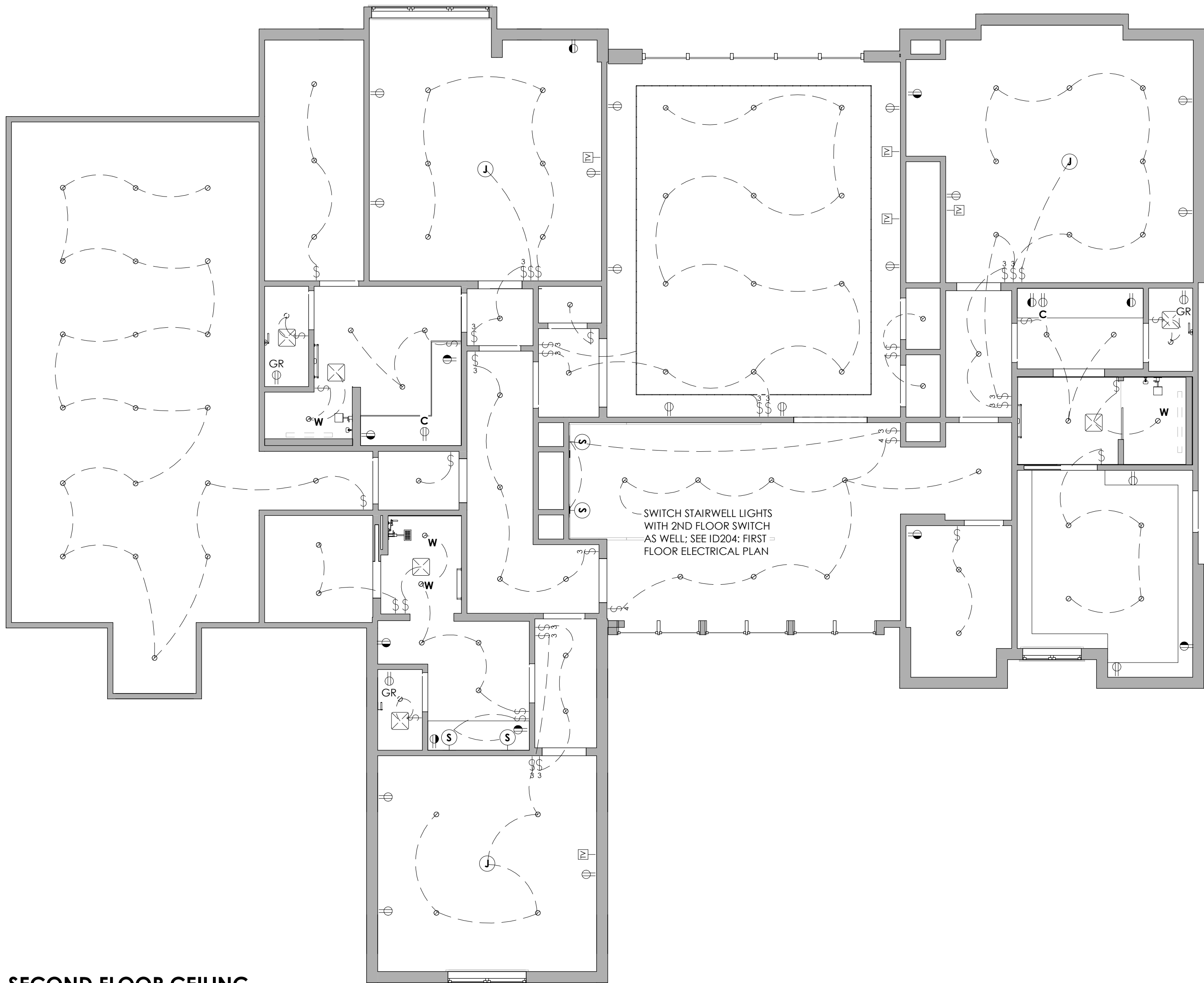
SECOND FLOOR CEILING PLAN
