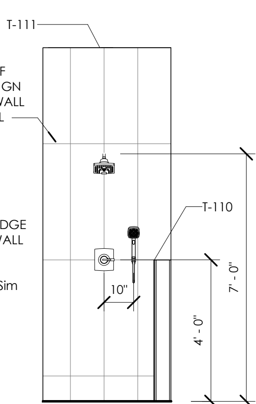
9 GUEST BATH 3 B 3/8" = 1'-0"
