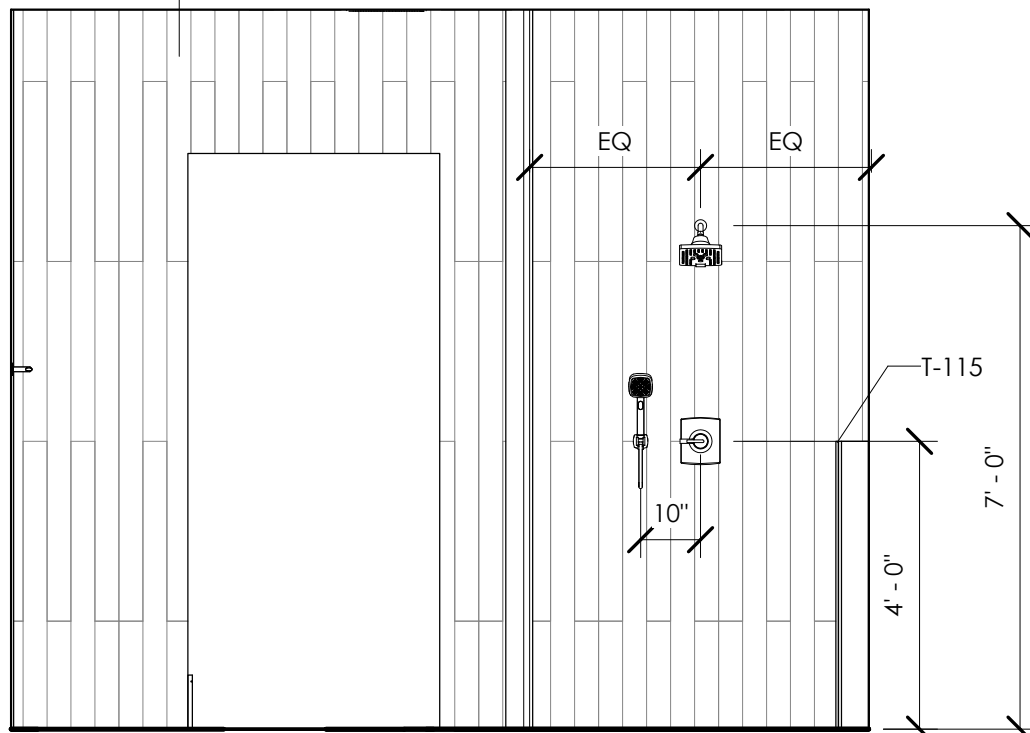
14 GUEST BATH 2 B 3/8" = 1'-0"
