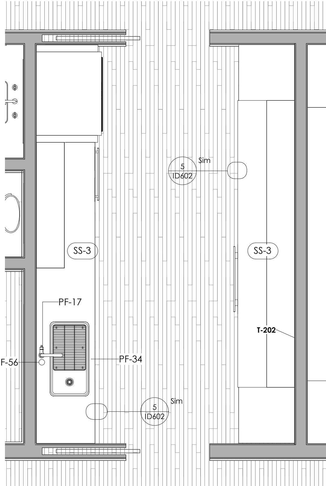
4 LEVEL 1 - SCULLERY 1/2" = 1'-0"
