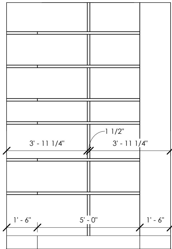
6 PANTRY C 3/8" = 1'-0"
