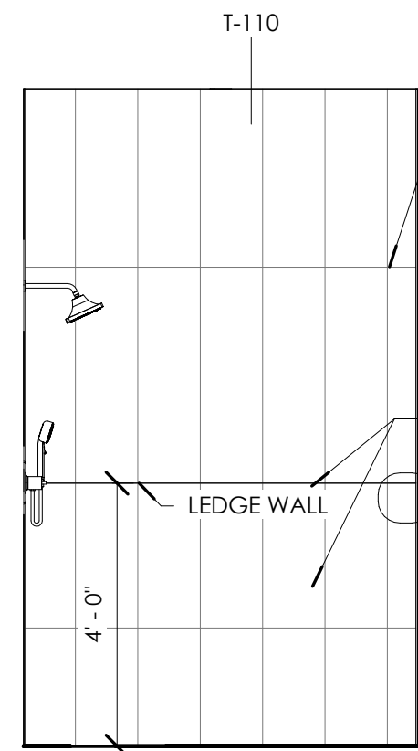
8 GUEST BATH 3 A 3/8" = 1'-0"
