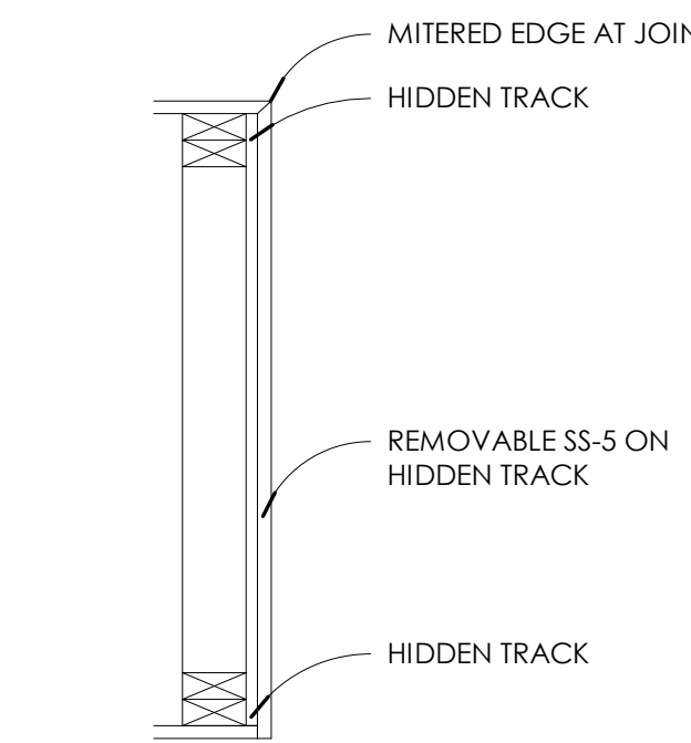
6 POWDER BATH VANITY DETAIL B 1" = 1'-0"
