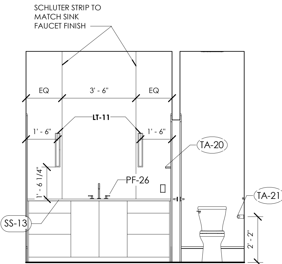
4 GUEST BATH A 3/8" = 1'-0"
