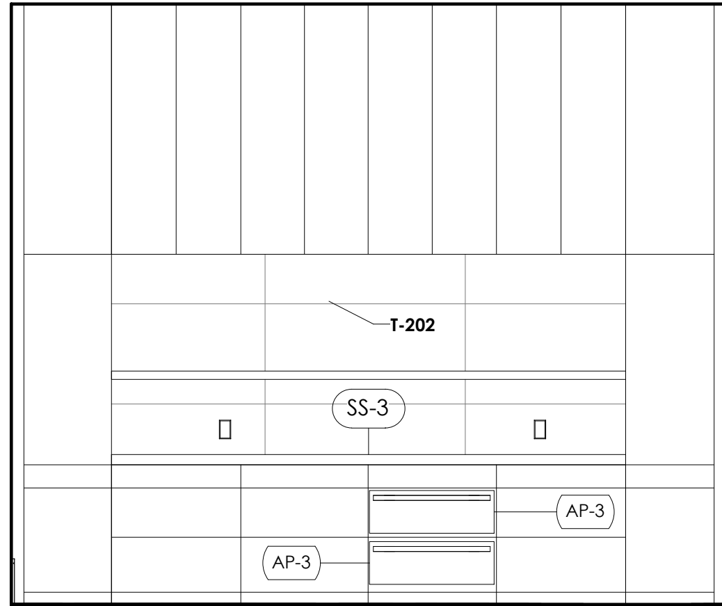
2 SCULLERY B 3/8" = 1'-0"
