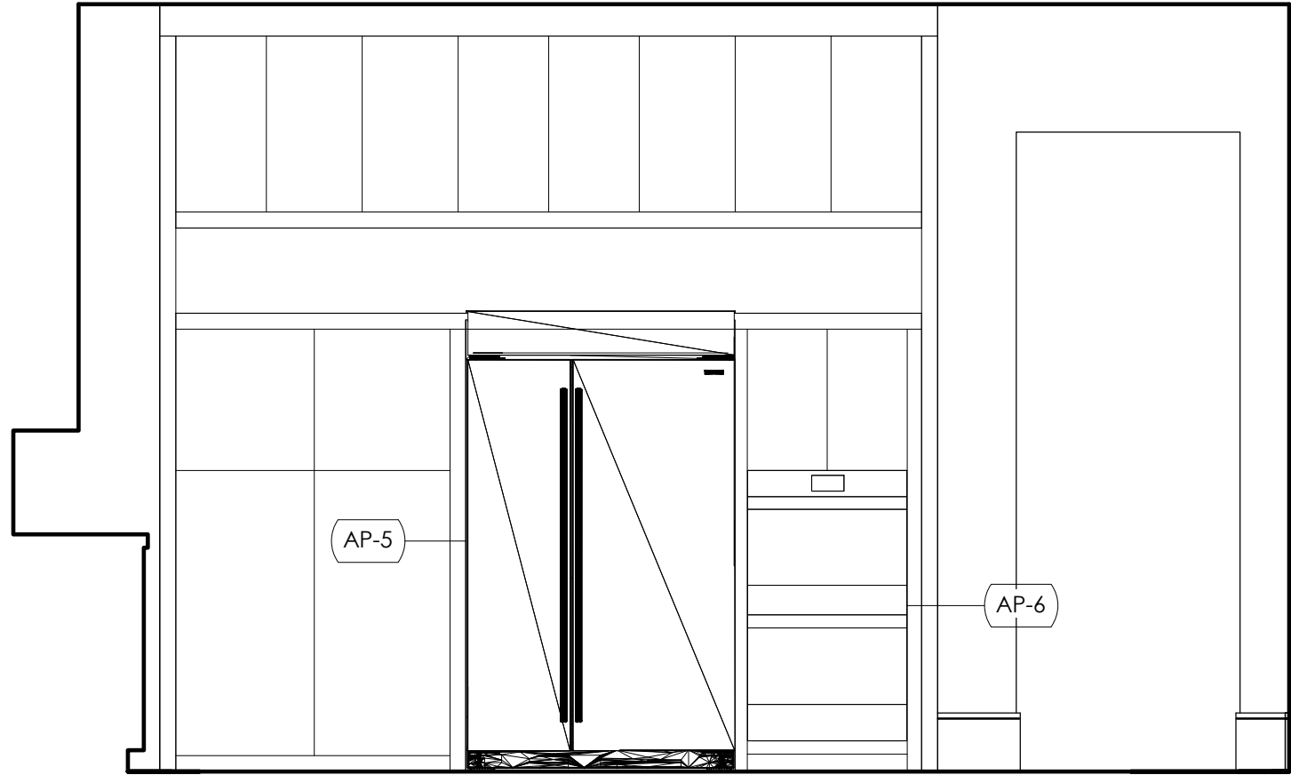
6 KITCHEN B 3/8" = 1'-0"
