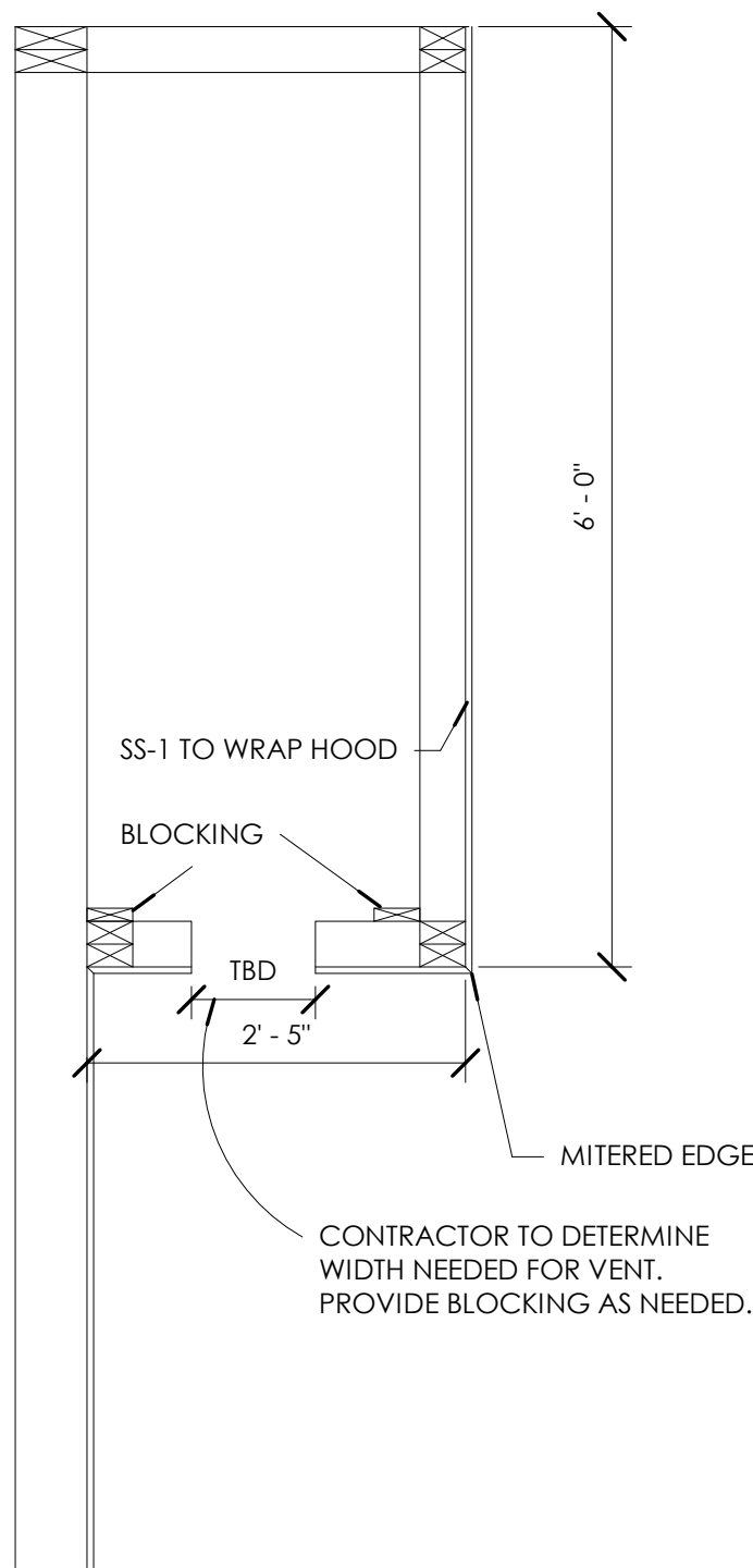
2 KITCHEN HOOD DETAIL 3/4" = 1'-0"
