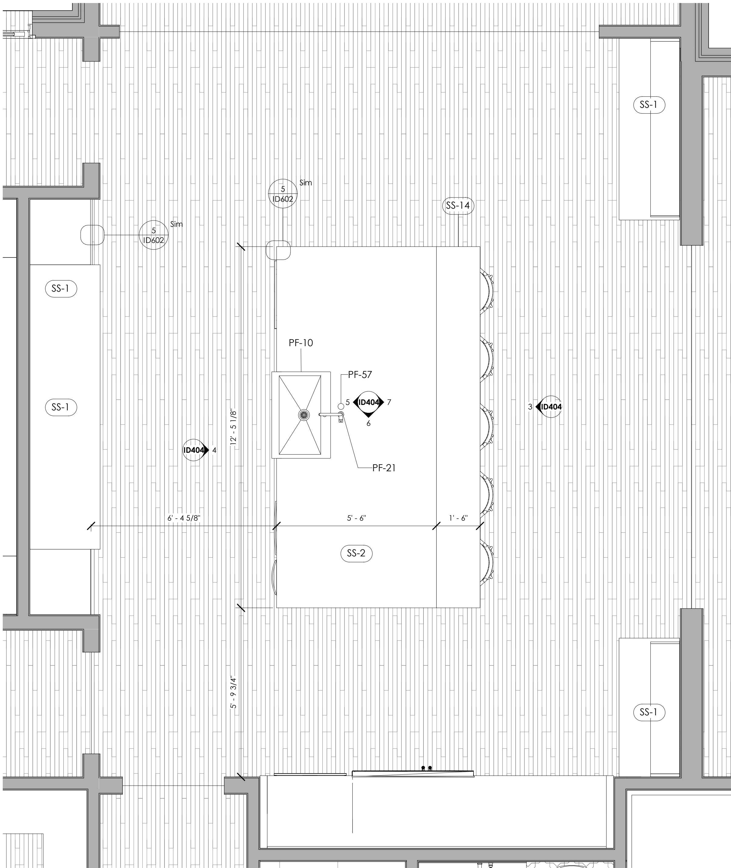
1 LEVEL 1 - KITCHEN 1/2" = 1'-0"
