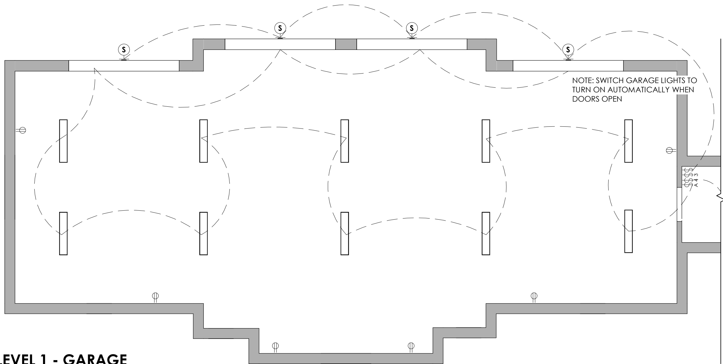
LEVEL 1 - GARAGE ELECTRICAL PLAN
