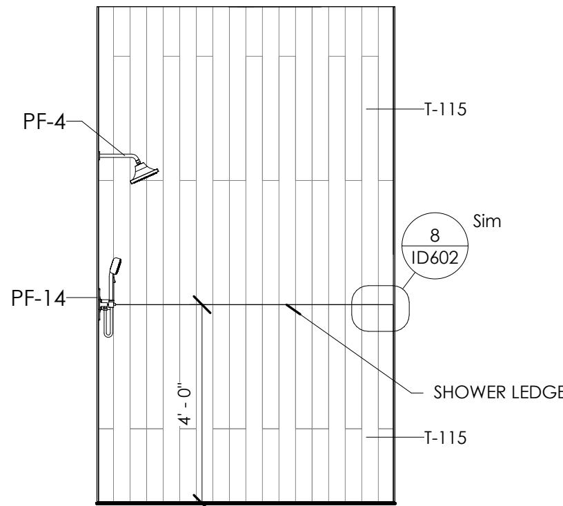
13 GUEST BATH 2 C 3/8" = 1'-0"
