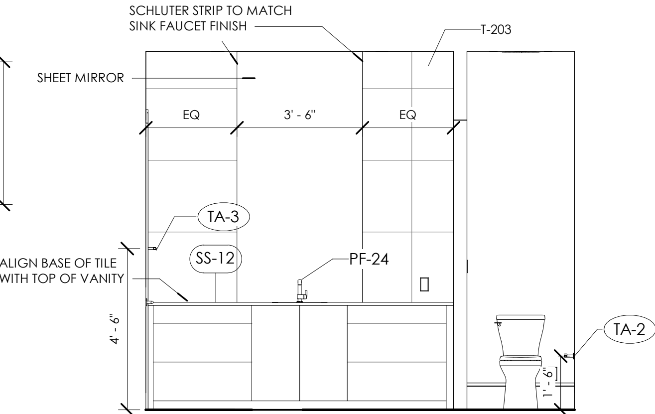
11 GUEST BATH 2 A 3/8" = 1'-0"
