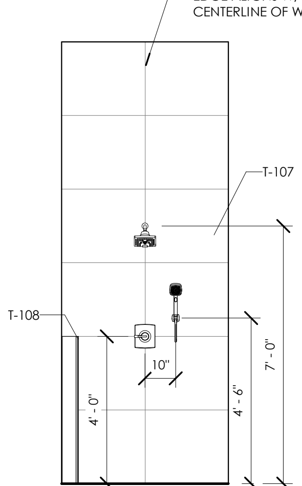
2 HIS BATH C 3/8" = 1'-0"
