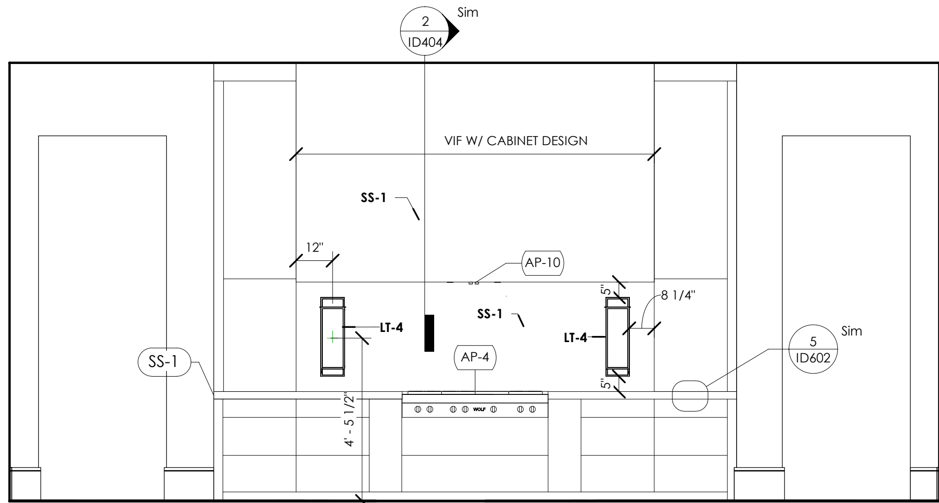
5 KITCHEN C 3/8" = 1'-0"
