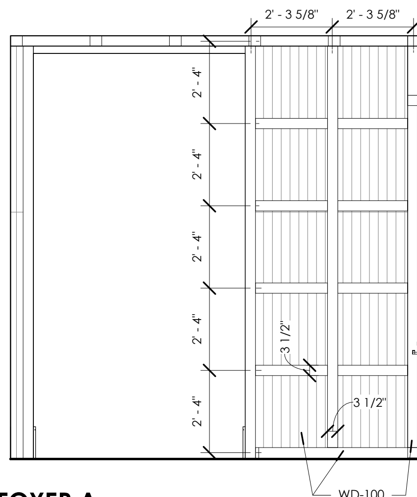
6 FOYER A 3/8" = 1'-0"
